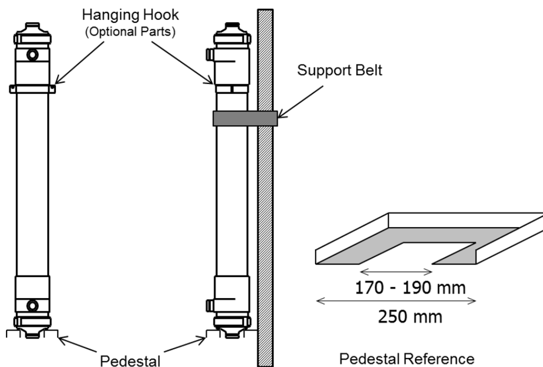
Fig. 2. Typical example of the membrane module installation
