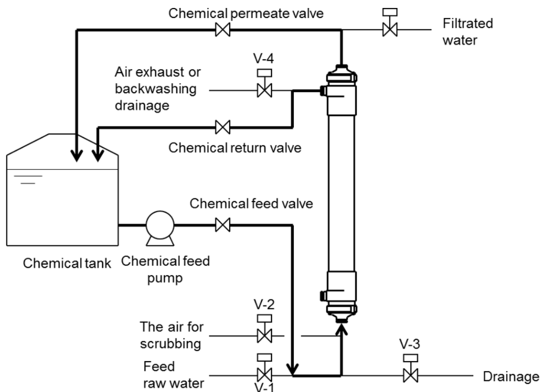
Fig. 9. Flow diagram for chemical cleaning
