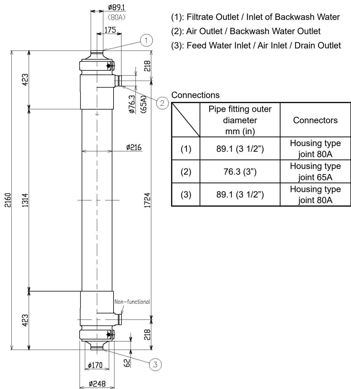
Fig. 1 Type: HFUG-2020HN
