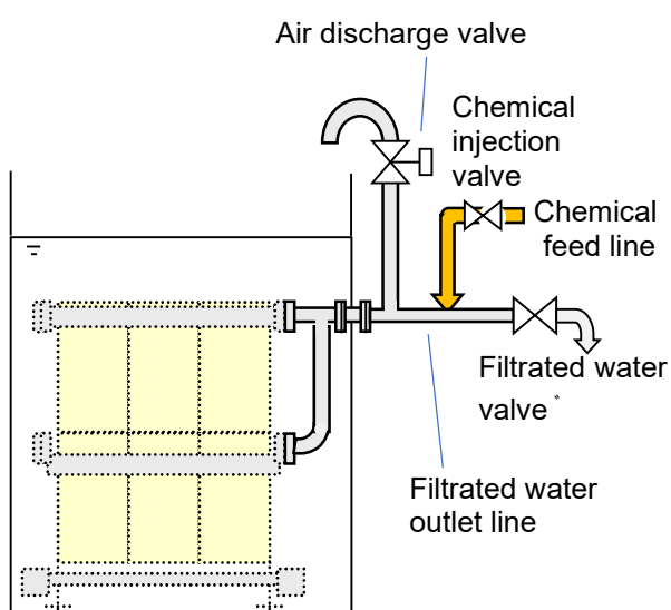
Figure IV-12: Downward Piping from MBR
