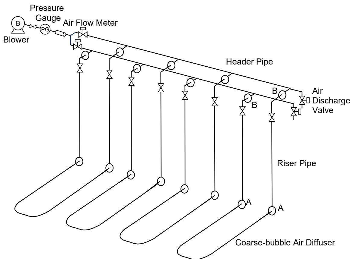
Figure IV-10: Coarse-bubble Air Diffuser Configuration Example (Per Header Pipe)
