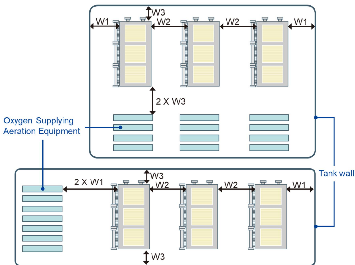
Figure IV-8: Membrane Module Layout in MBR Tank with Other Aeration Equipment (Top View)
