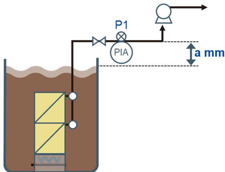
Figure IV-4: TMP Measurement & Calculation (Stable Liquid Level)
