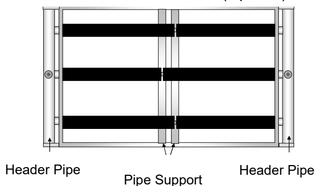
Aeration block ABL150-F (top view)
