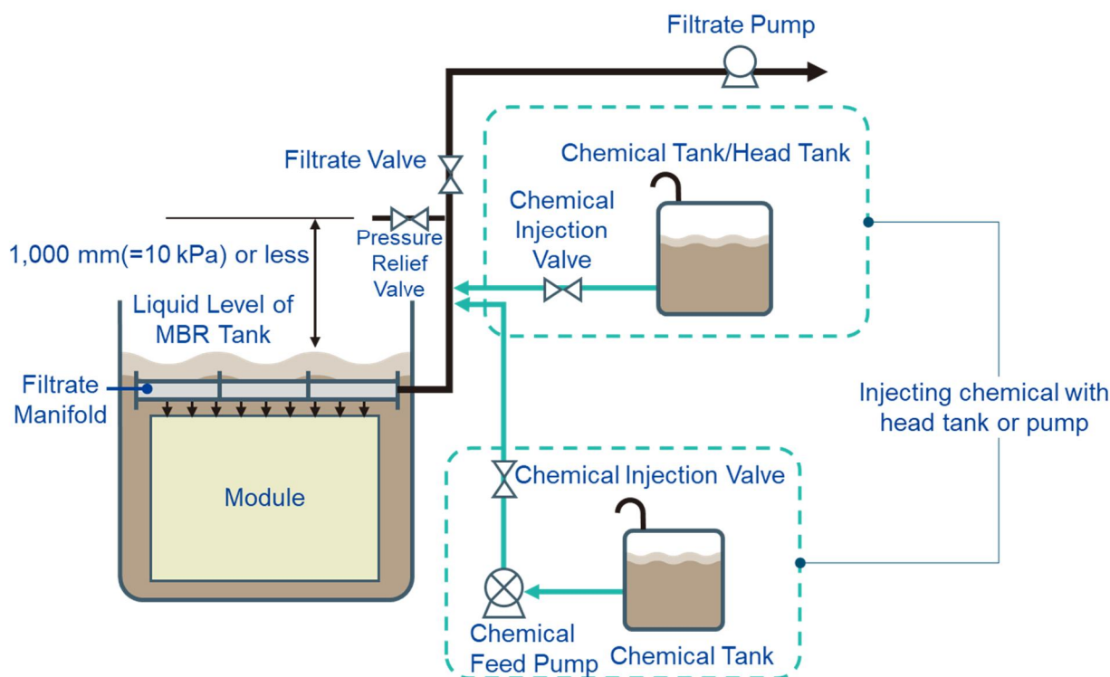
Figure VIII-3: Chemical Cleaning Flow Diagram (Filtrate Upward Discharge Piping)
