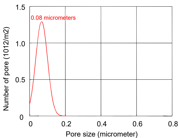
Figure I-7: Pore Size
