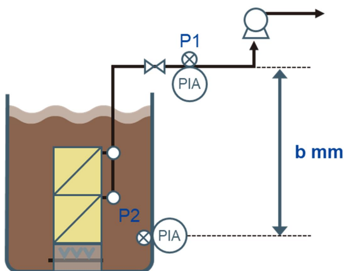
Figure IV-5: TMP Measurement & Calculation (Fluctuating Liquid Level)
