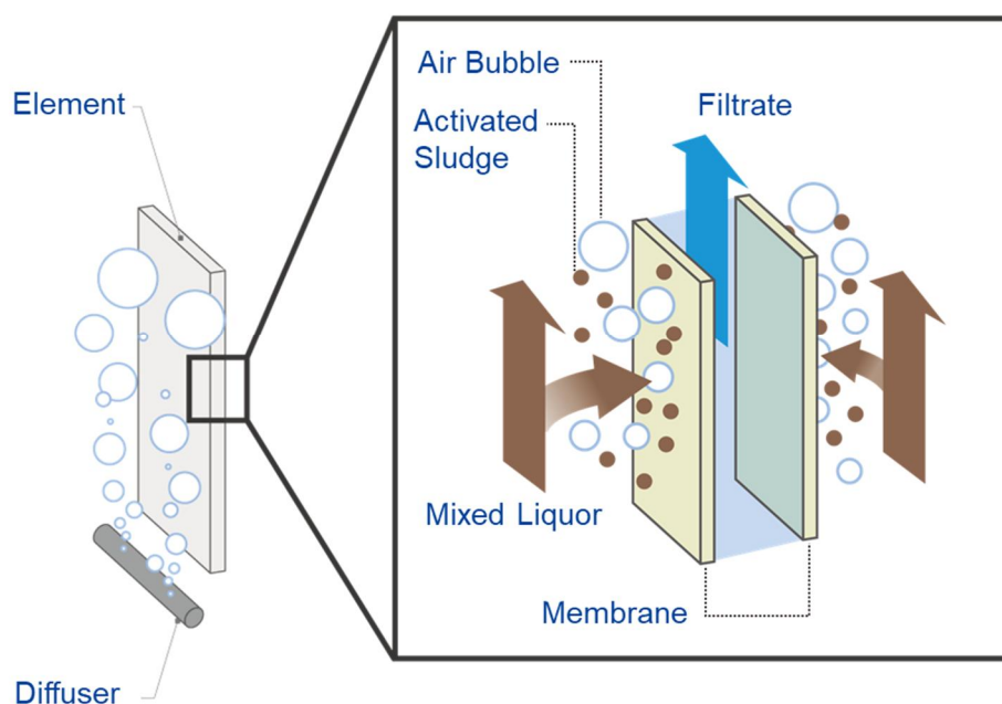
Figure I-5: Filtration Principle of Activated Sludge
