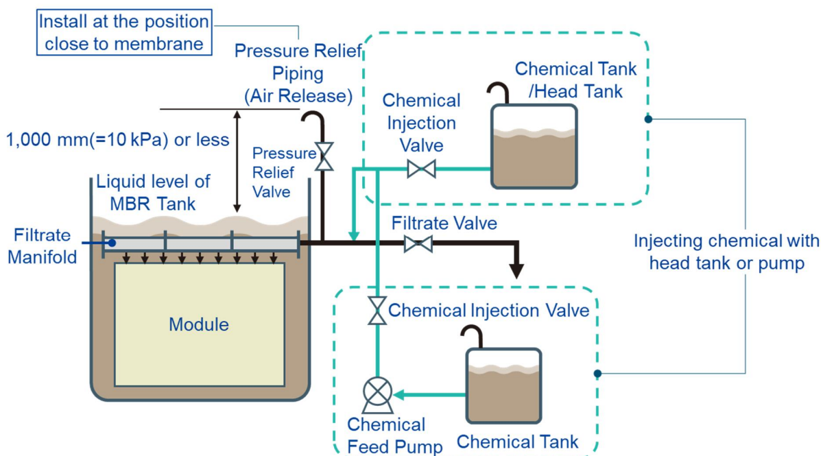
Figure VIII-2: Chemical Cleaning Flow Diagram (Filtrate Downward Discharge Piping)
