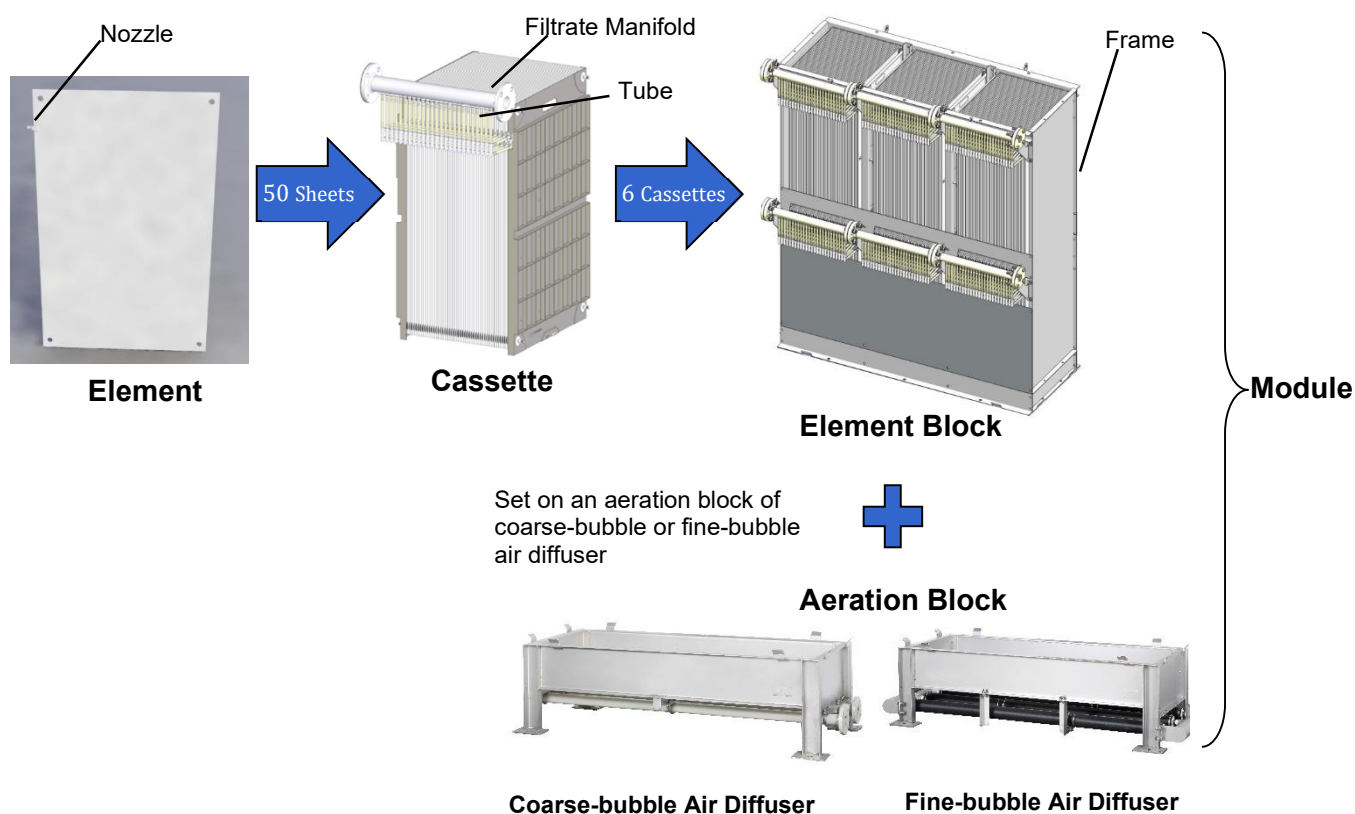
Figure I-3: Components and Appearance of Module (NHP210-300S: 3 cassettes x 2 stacks)
