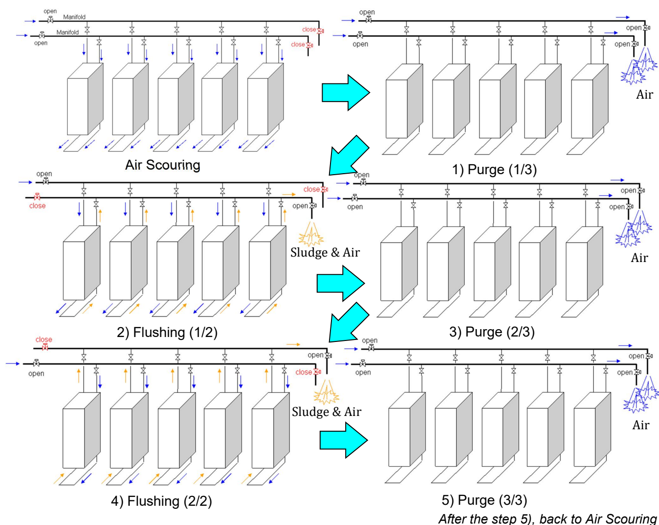
Figure VIII-1: Air Diffuser Cleaning Procedure for Multiple Modules
