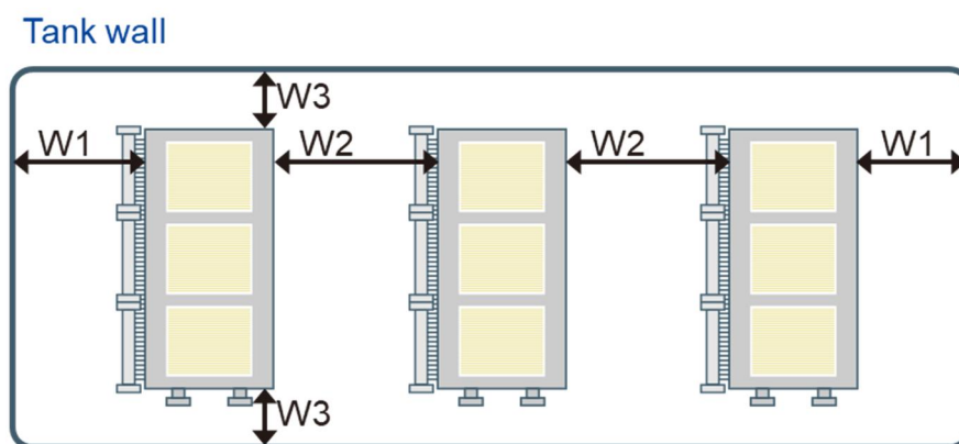
Figure IV-6b: Membrane Module Layout in MBR Tank (top view)
