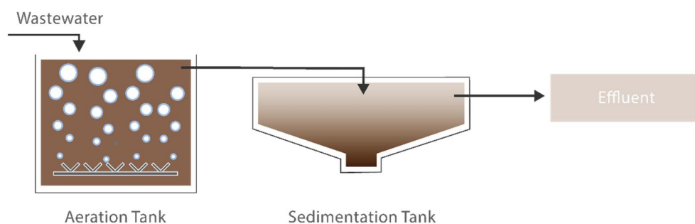
Figure I-1: CAS Flow
