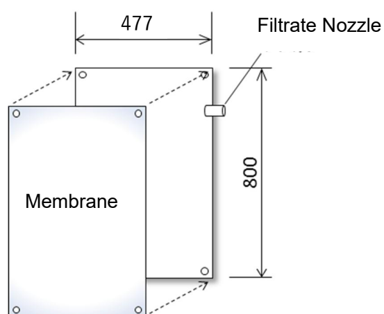
Figure I-4: Structure of Element
