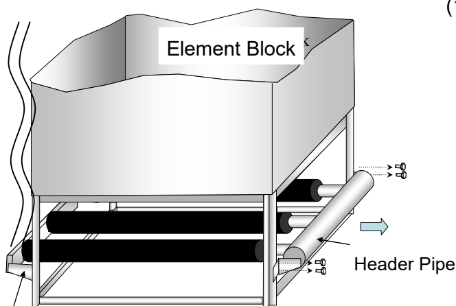
Pipe Support
