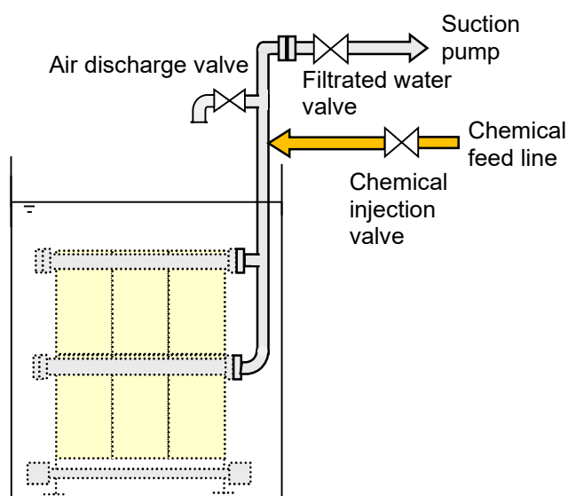
Figure IV-13: Upward Piping from MBR
