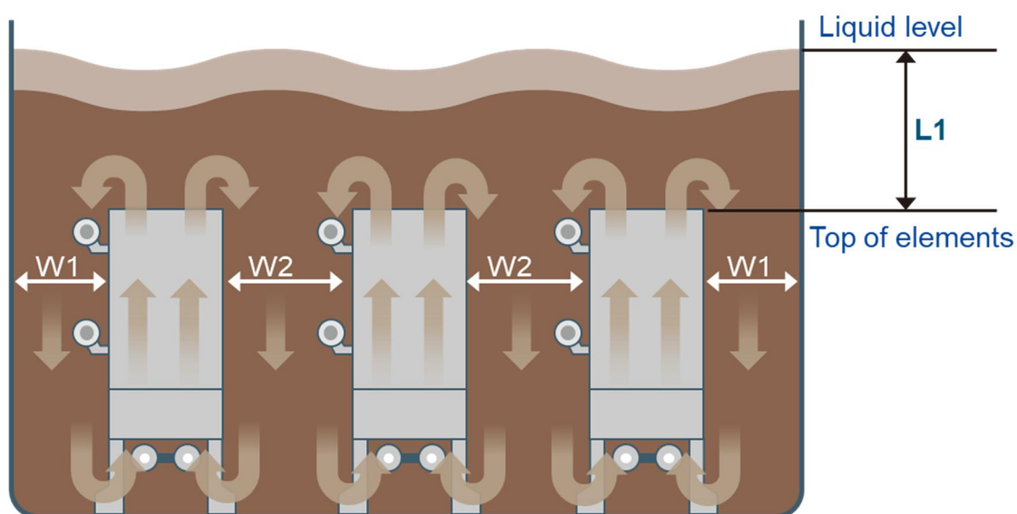
Figure IV-6a: Membrane Module Layout in MBR Tank (side view)
