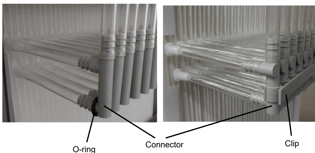
Figure III-2: Tube Set Appearance
