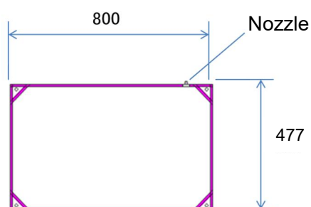
Figure III-1: Element Appearance (mm)
