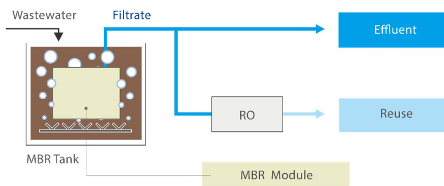
Figure I-2: MBR Flow
