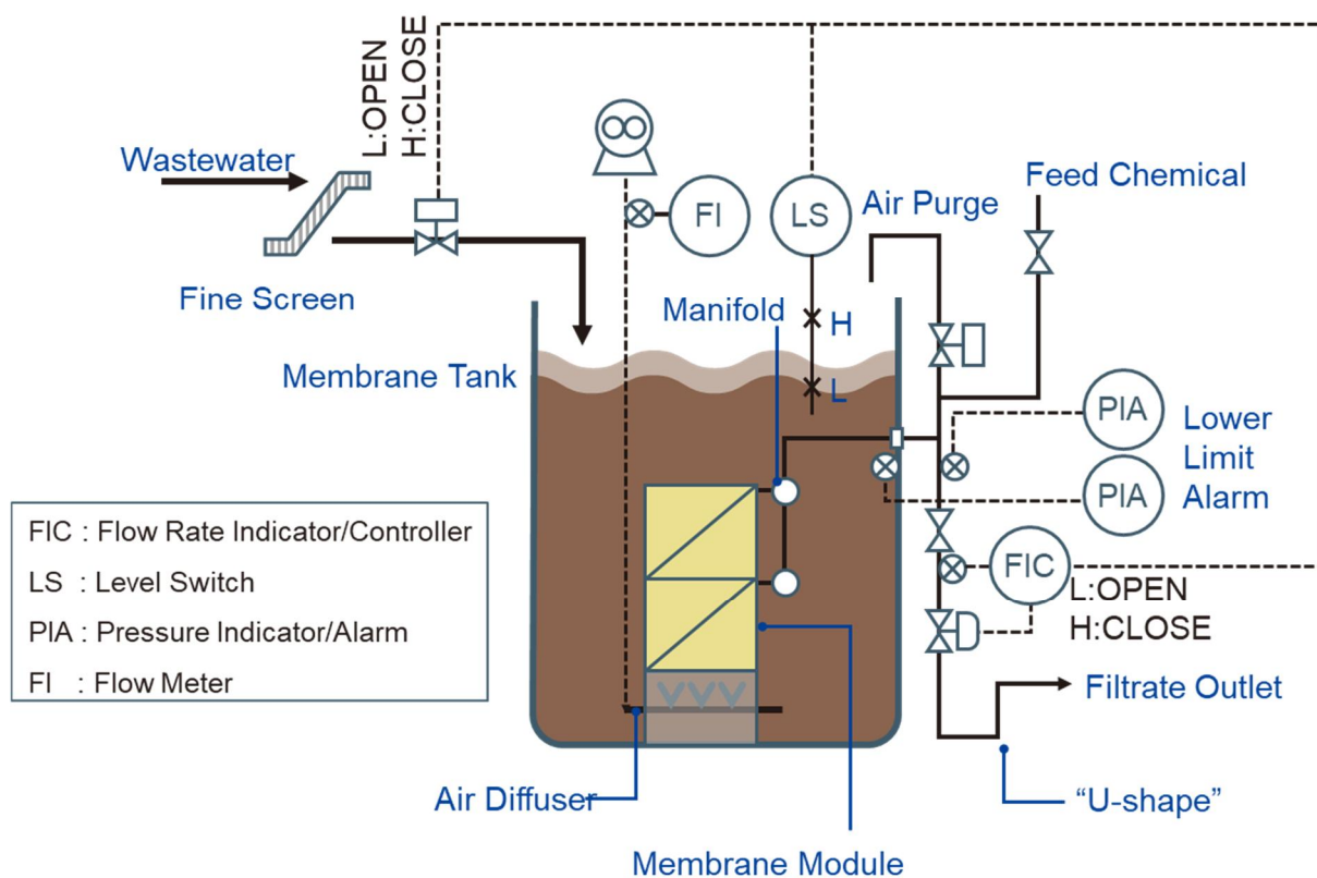
Figure IV-2: Schematic Flow Diagram for Gravity Filtration
