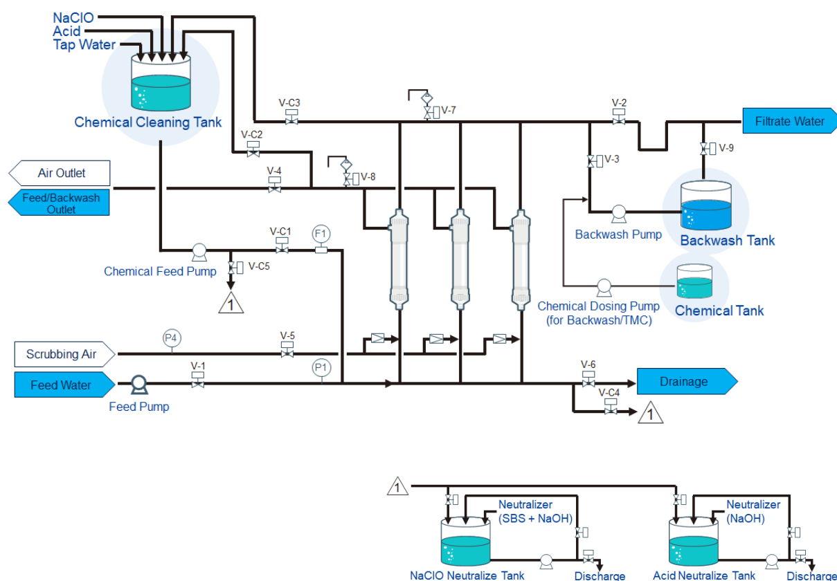
Figure 6-1: UF Plant Configuration
