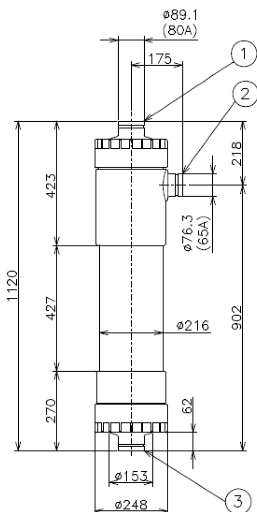
Figure 5.3-1: HFUG-1020AN
