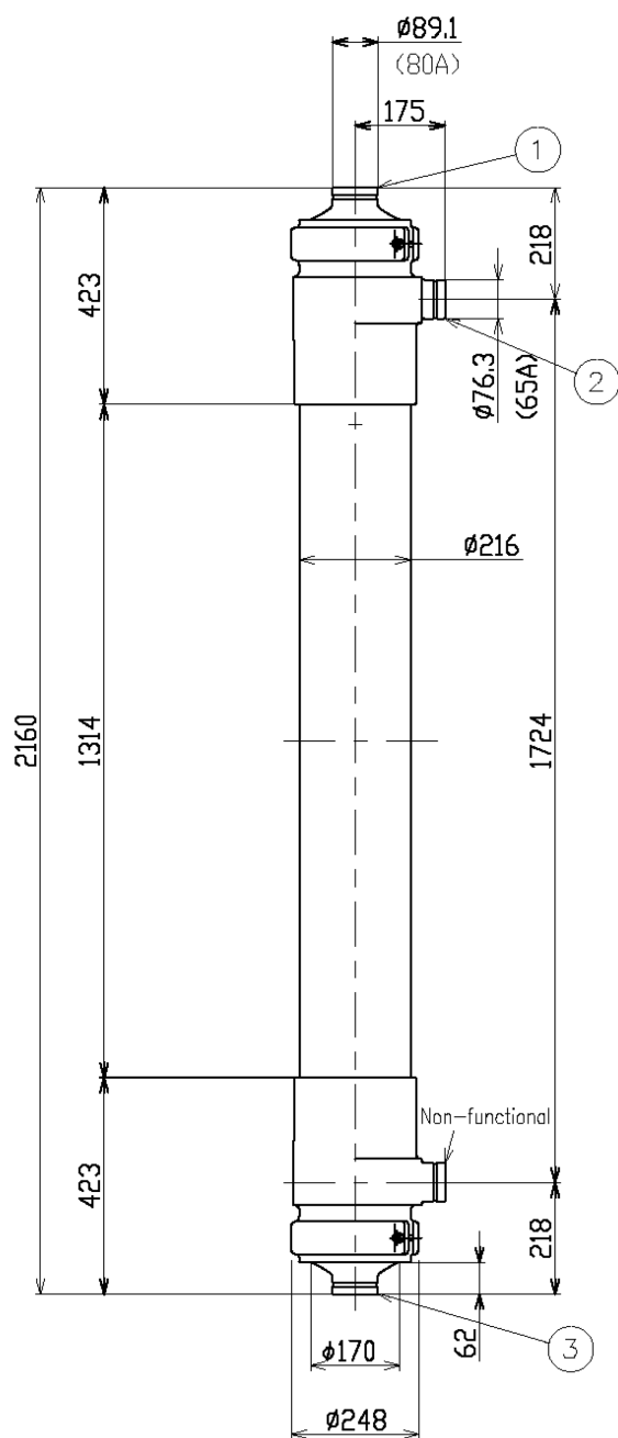
Figure 5.2-1: HFUG-2020HN
