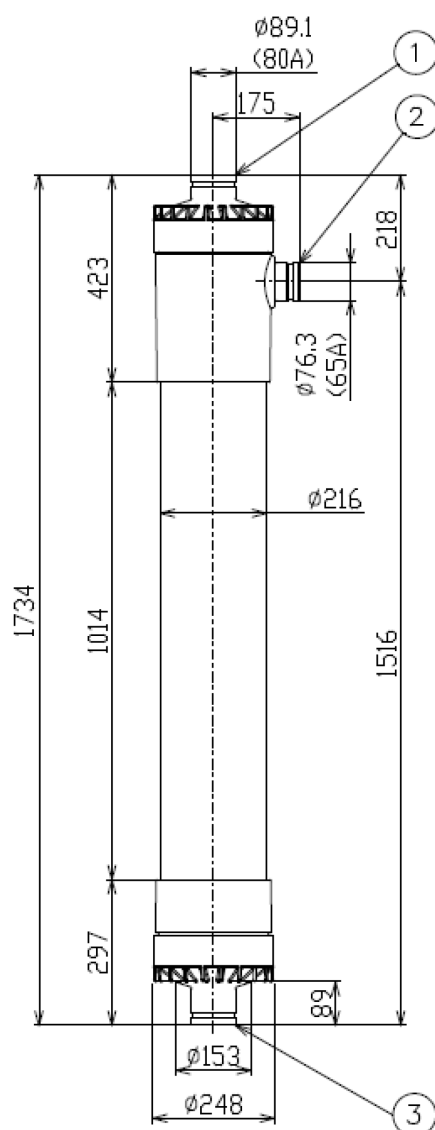
Figure 5.4-1: HFUG-L1720AN
