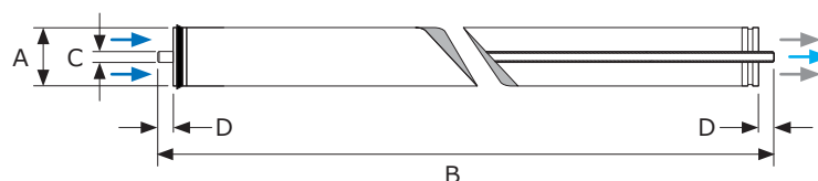
図2: TMH20A-400C, TMH20A-440C
