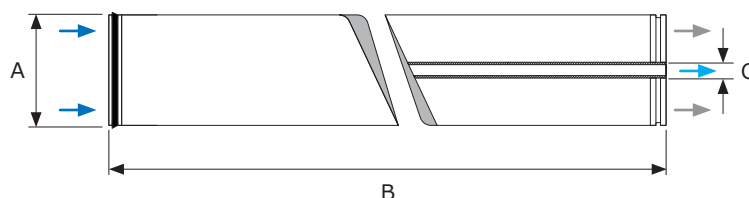
図2: TMH20A-400C, TMH20A-440C
